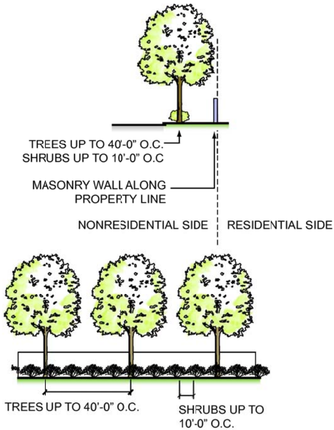
18-95.16.1 SCREENING WALL
