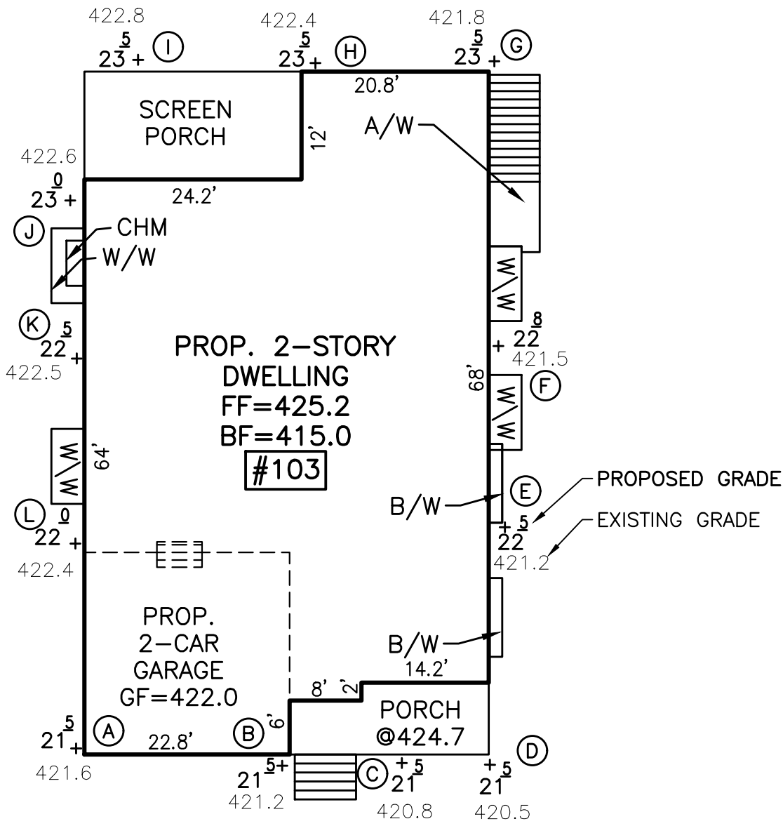
PROPOSED AND EXISTING GRADES (SCALE:1":15')
