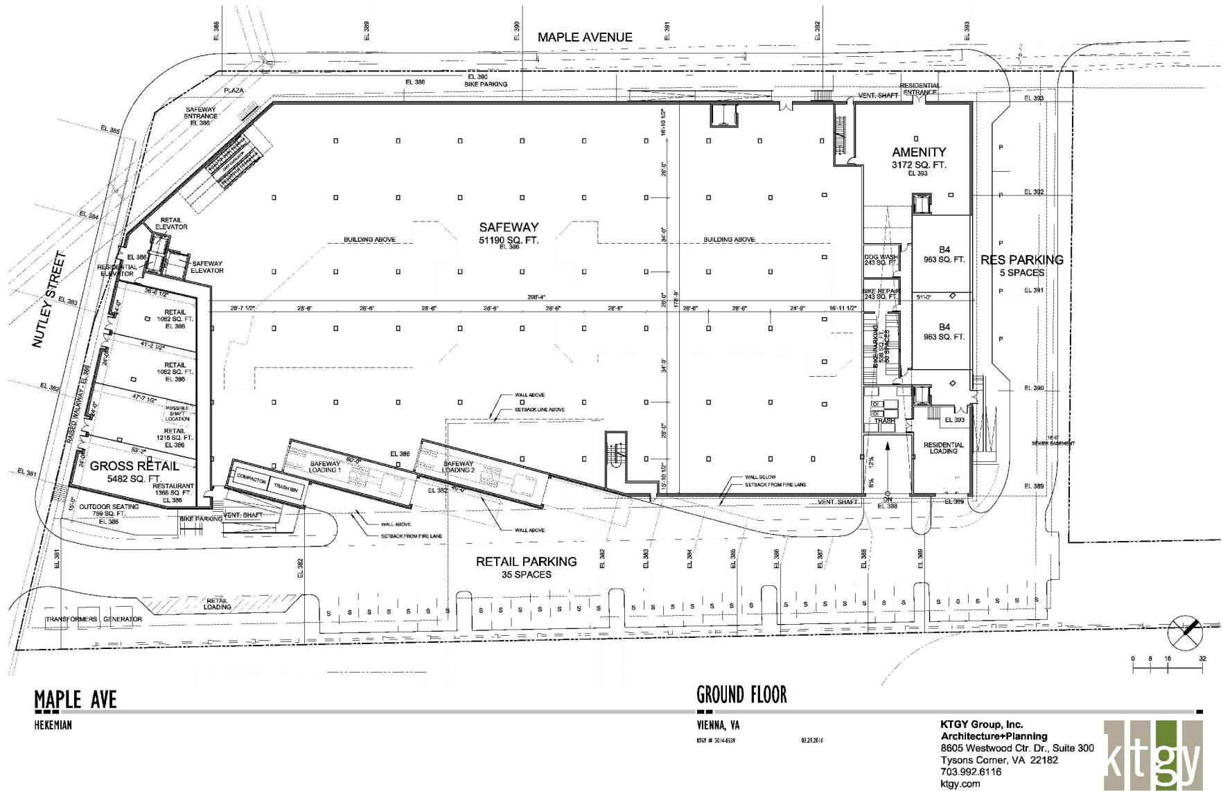
Attachment II Ground Floor Layout
