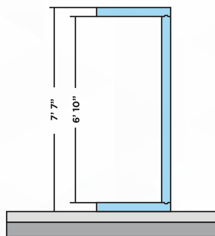
SIDE VIEW WITH FLOOR
