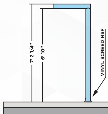
SIDE VIEW WITH NO FLOOR (COOLER ONLY)
