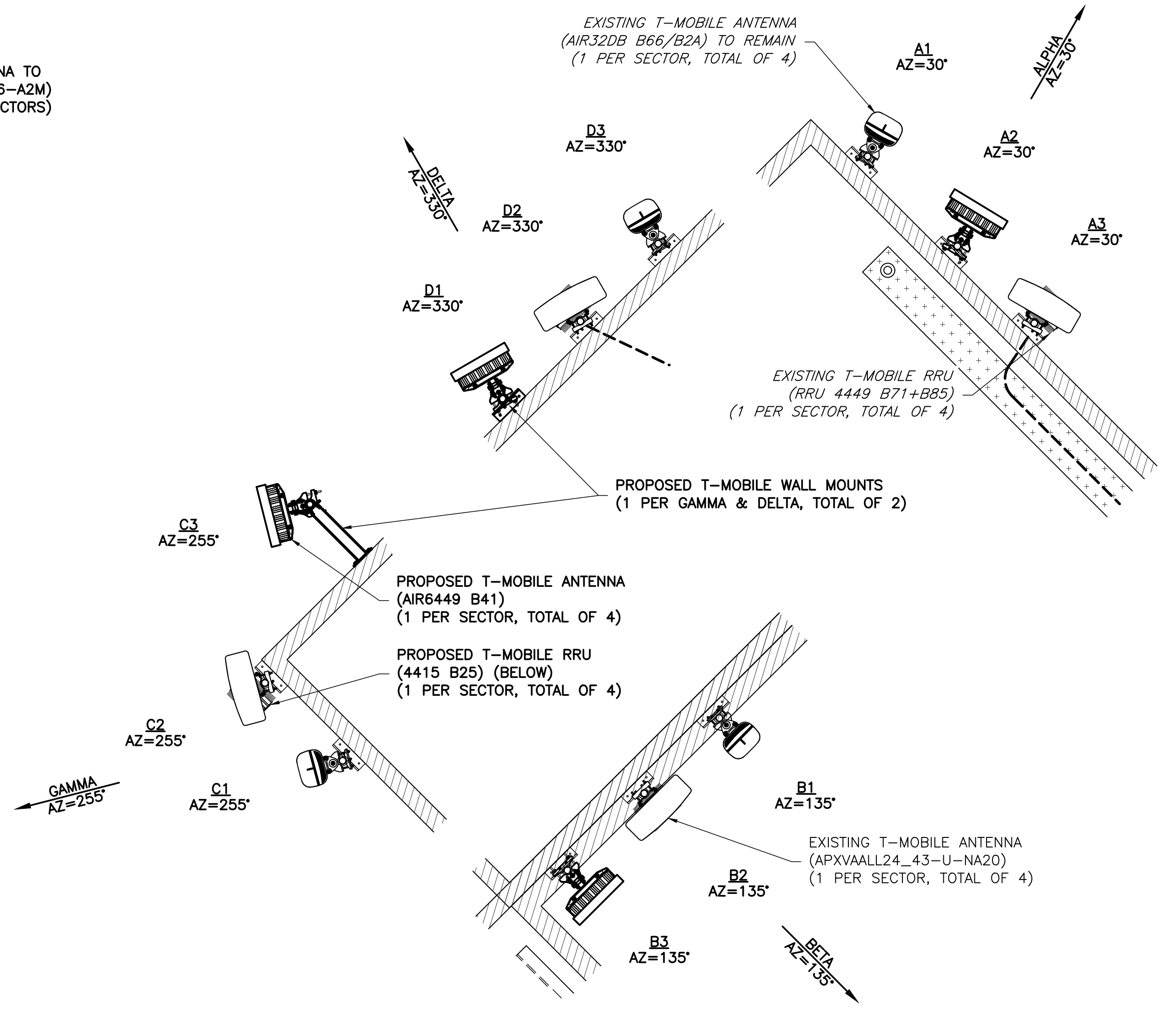
2 PROPOSED ANTENNA ORIENTATION PLAN A-1 NTS
