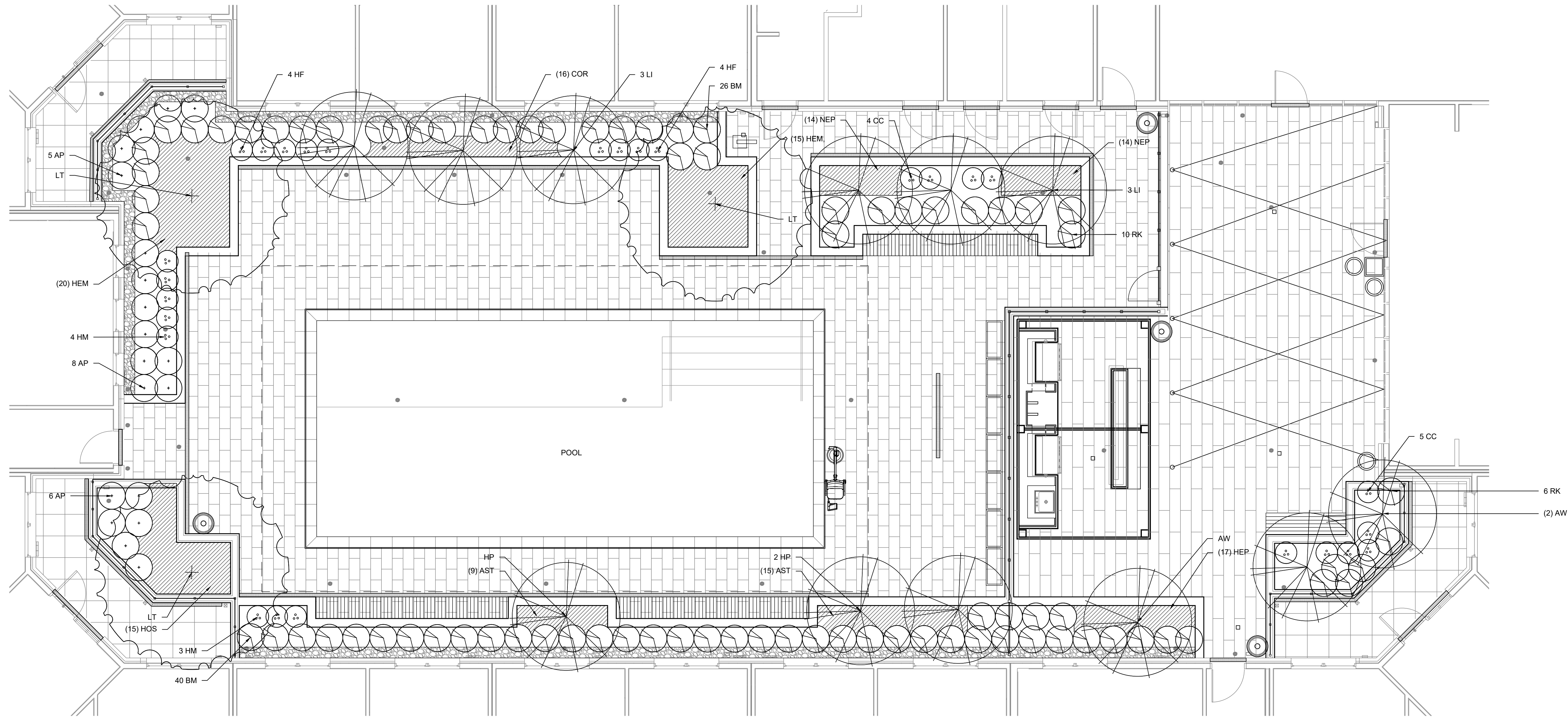
1 PLANTING PLAN - COURTYARD EAST 3/16"=1'-0"
