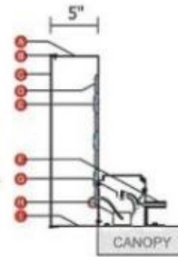
SECTION - FACE-LIT RACEWAY NTS
