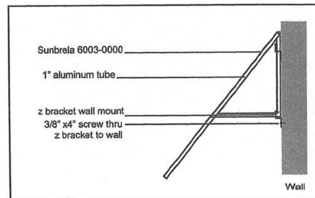
SIGN SPECS (materials & mounting details)
