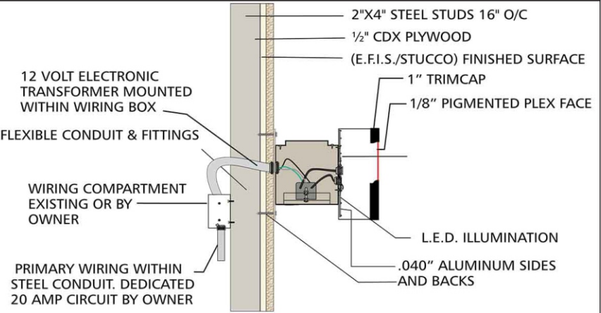
LED RACEWAY MOUNT TYPICAL - NOT TO SCALE
