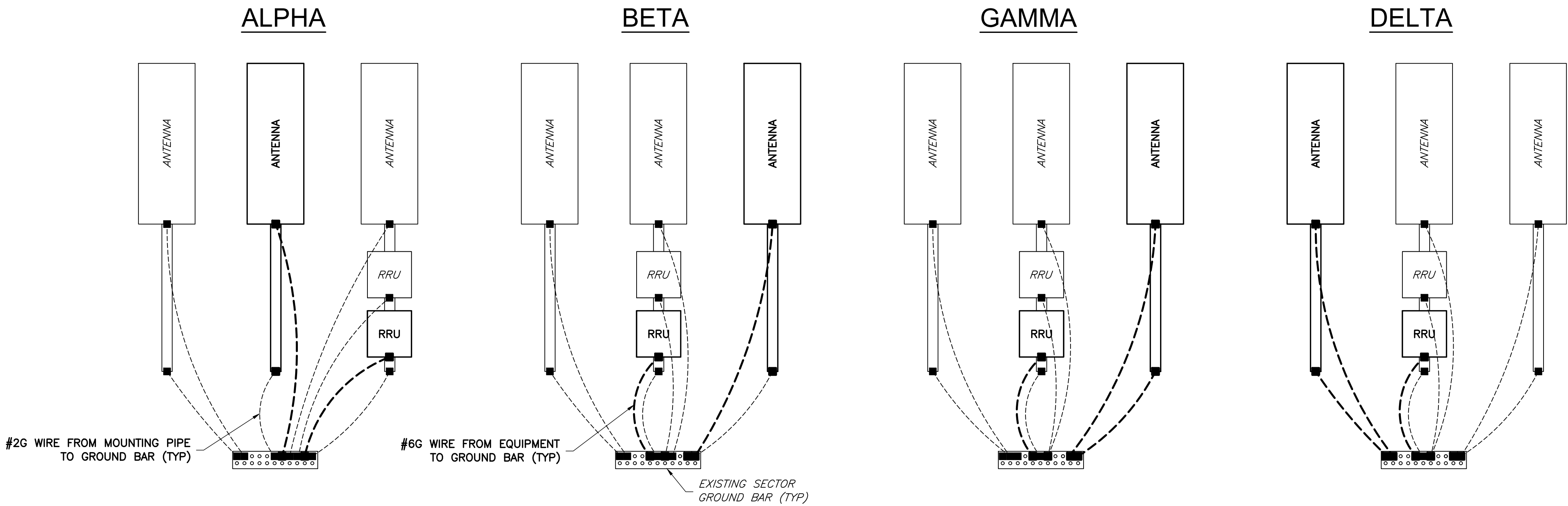
1 ANTENNA GROUNDING DETAIL G-1 NTS
