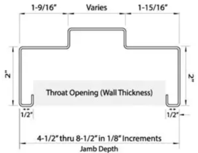
Storage Room HM Double Door Jamb Detail
