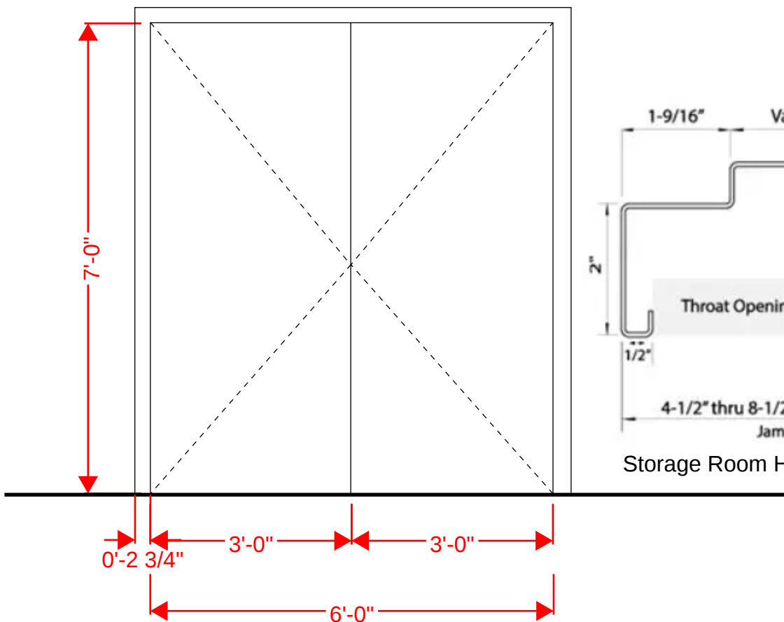
Storage Room HM Double Door Elevation
