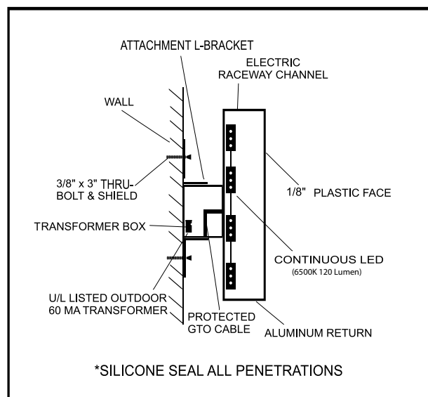
LETTER / RACEWAY INSTALLATION DETAIL NO SCALE
