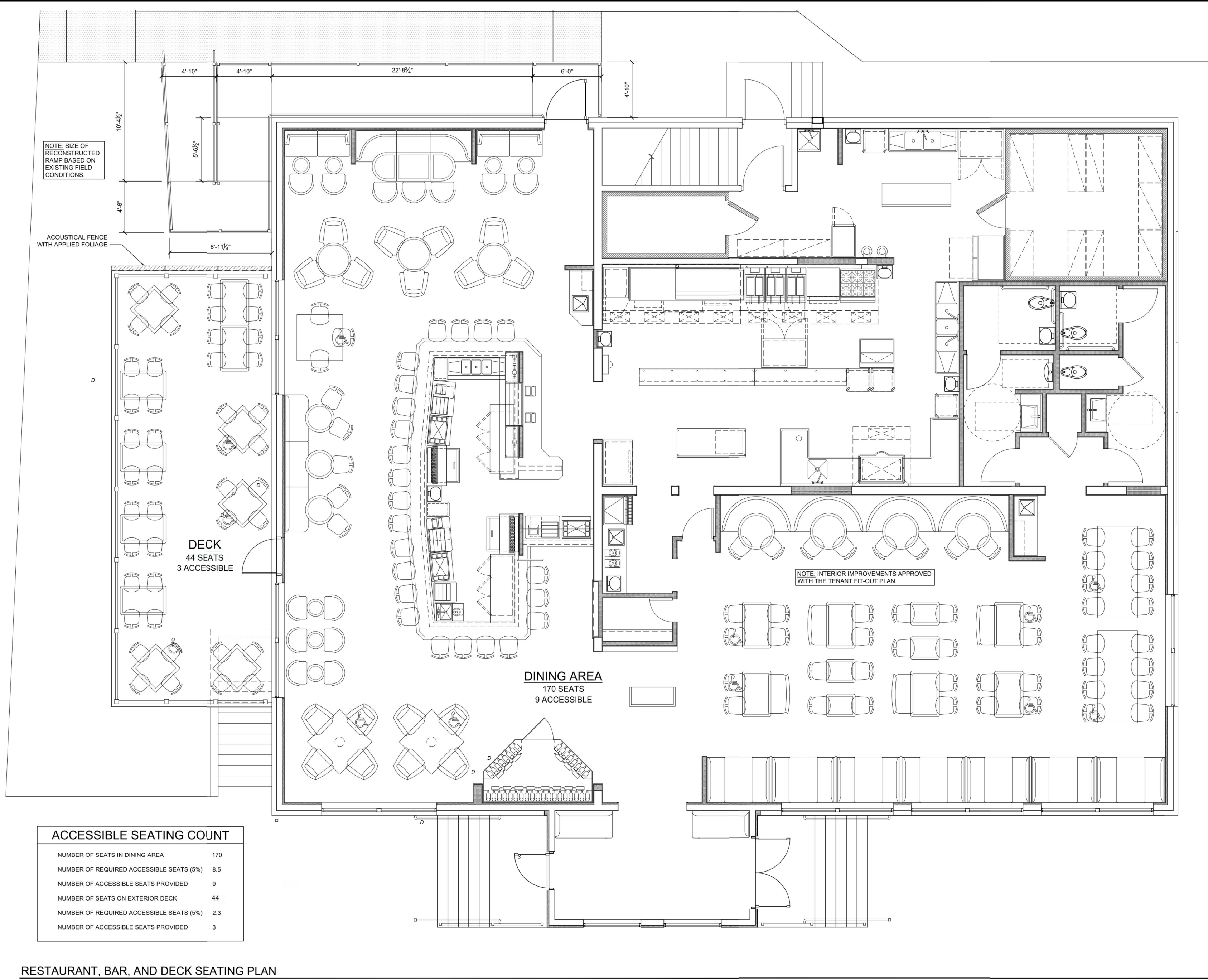
RESTAURANT, BAR, AND DECK SEATING PLAN SCALE: 1/4" = 1'-0"
