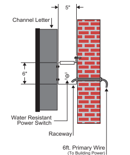
RACEWAY SIDE VIEW
