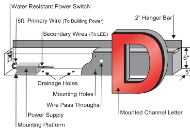
RACEWAY FRONT VIEW
