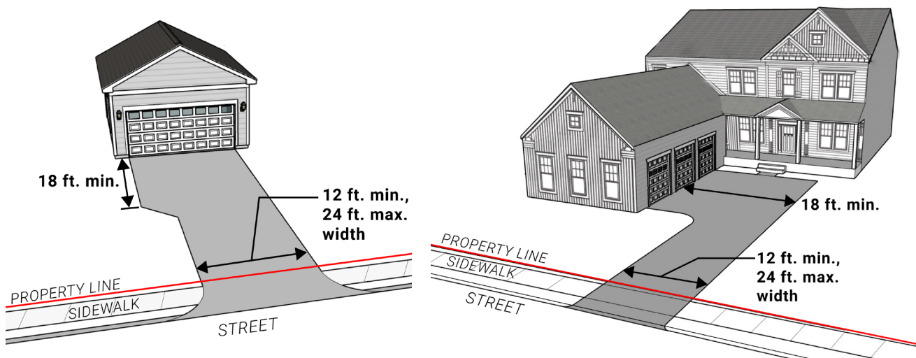
FIGURE 4A.5 Driveway standards
