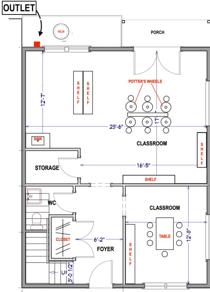
1st Floor
