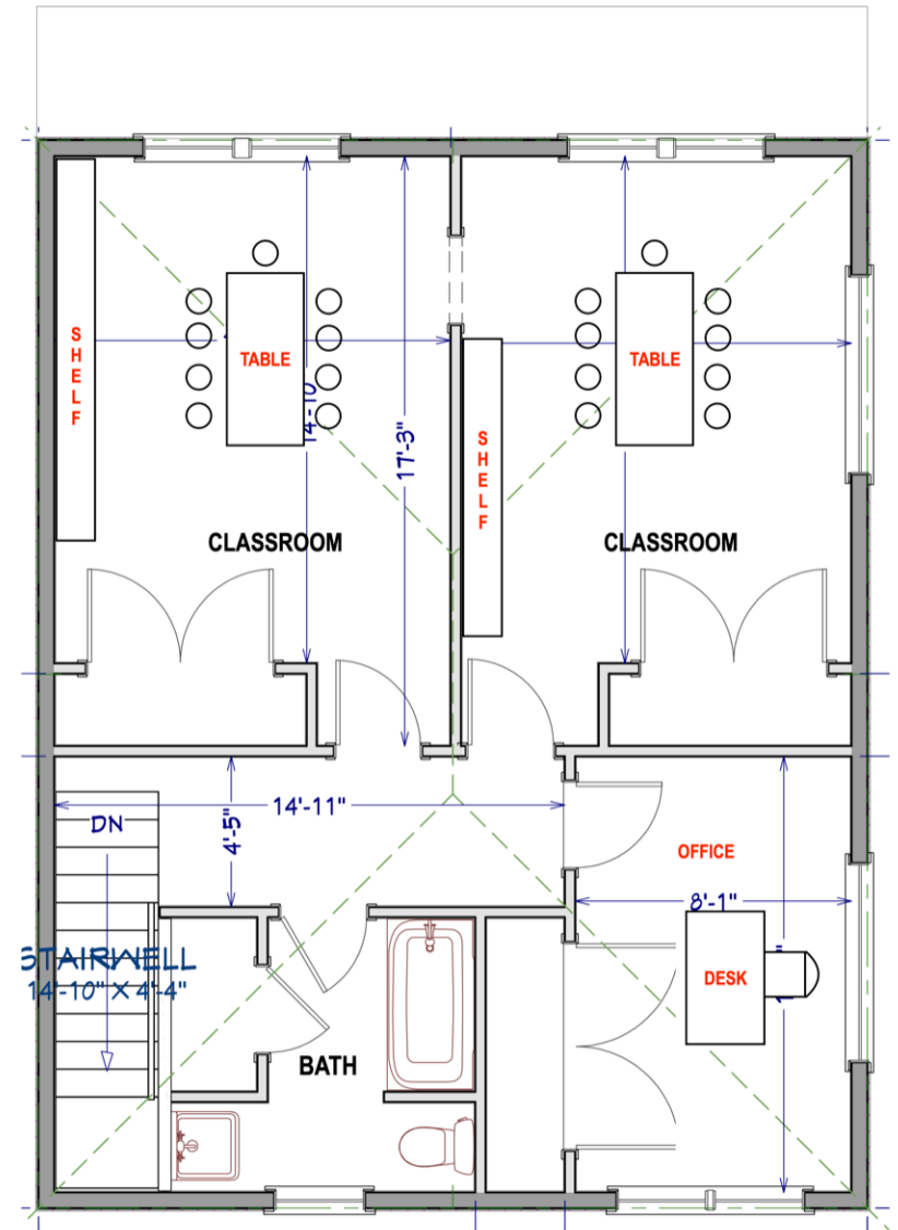
2nd Floor
