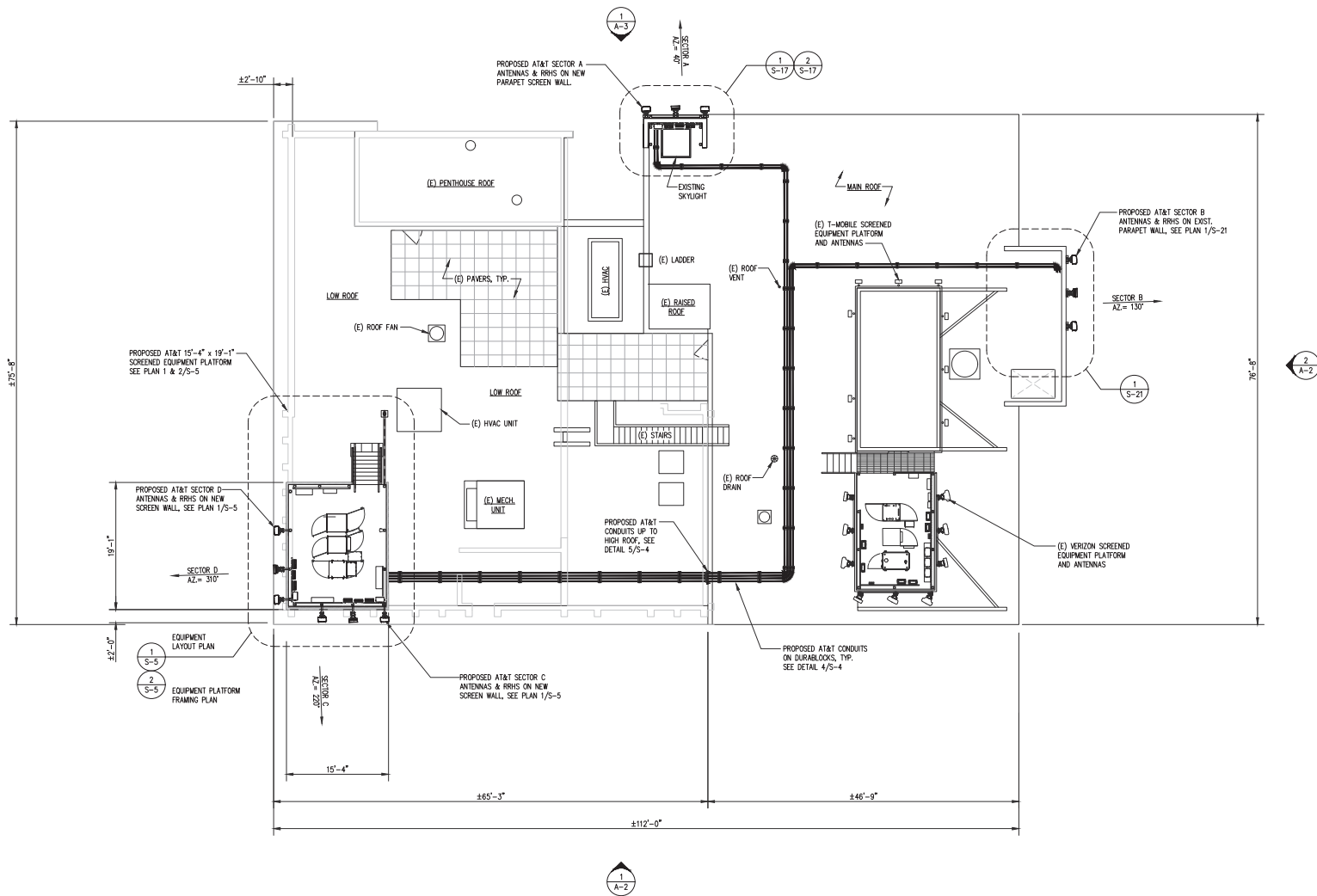
ROOF AND EQUIPMENT LOCATION PLAN SCALE: 1/8"=1'-0"
