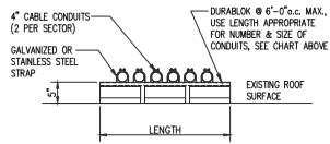
CABLE CONDUIT SUPPORT DETAIL
