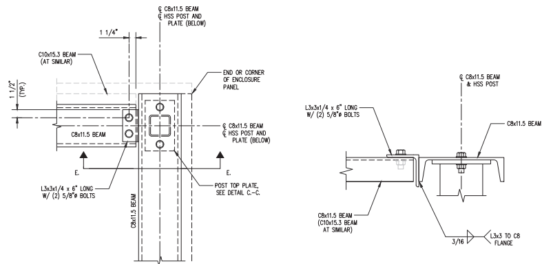
PLAN DETAIL SCALE: 1 1/2"=1'-0"
