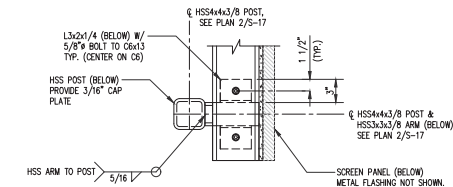
PLAN C-C.
