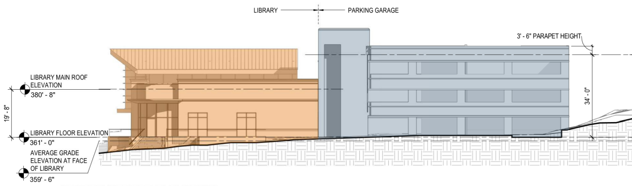
CENTER STREET ELEVATION NOT TO SCALE
