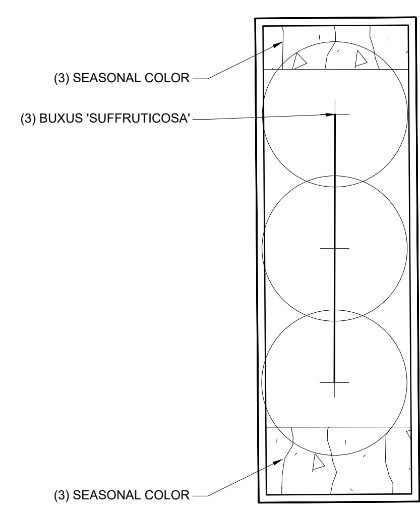
3 PLANTER TYPE 1 PLAN L6.03 Scale: 1" = 1'
