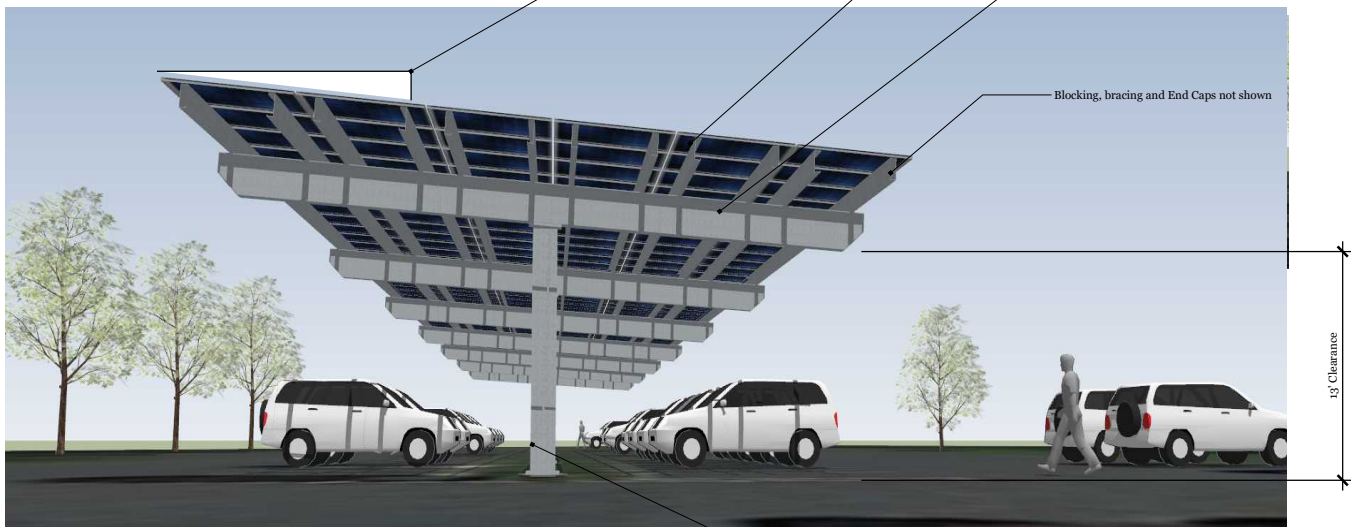
Base Plate flush with grade. Above ground pilasters as required to level canopy along length
