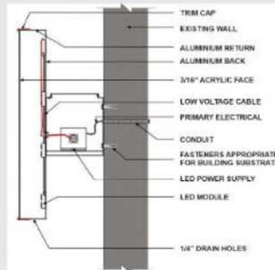
Standard Face Lit - LED Illuminated w/ Raceway
