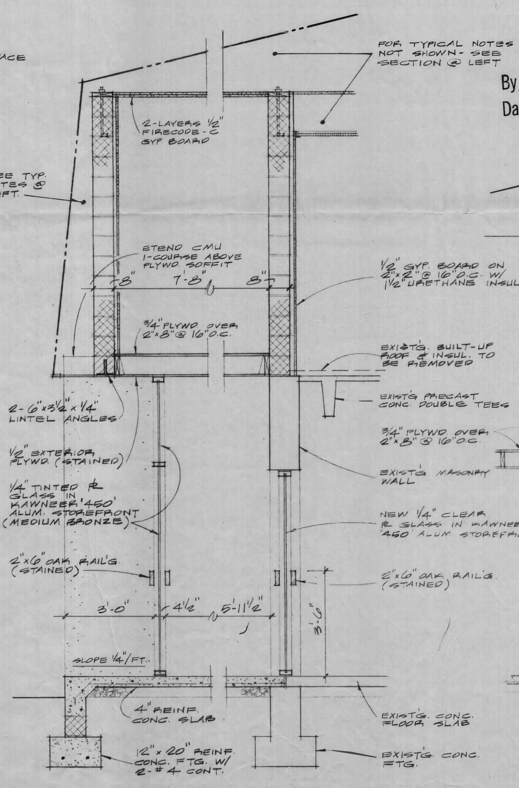
SECTION B 1/2" = 1'-0"
