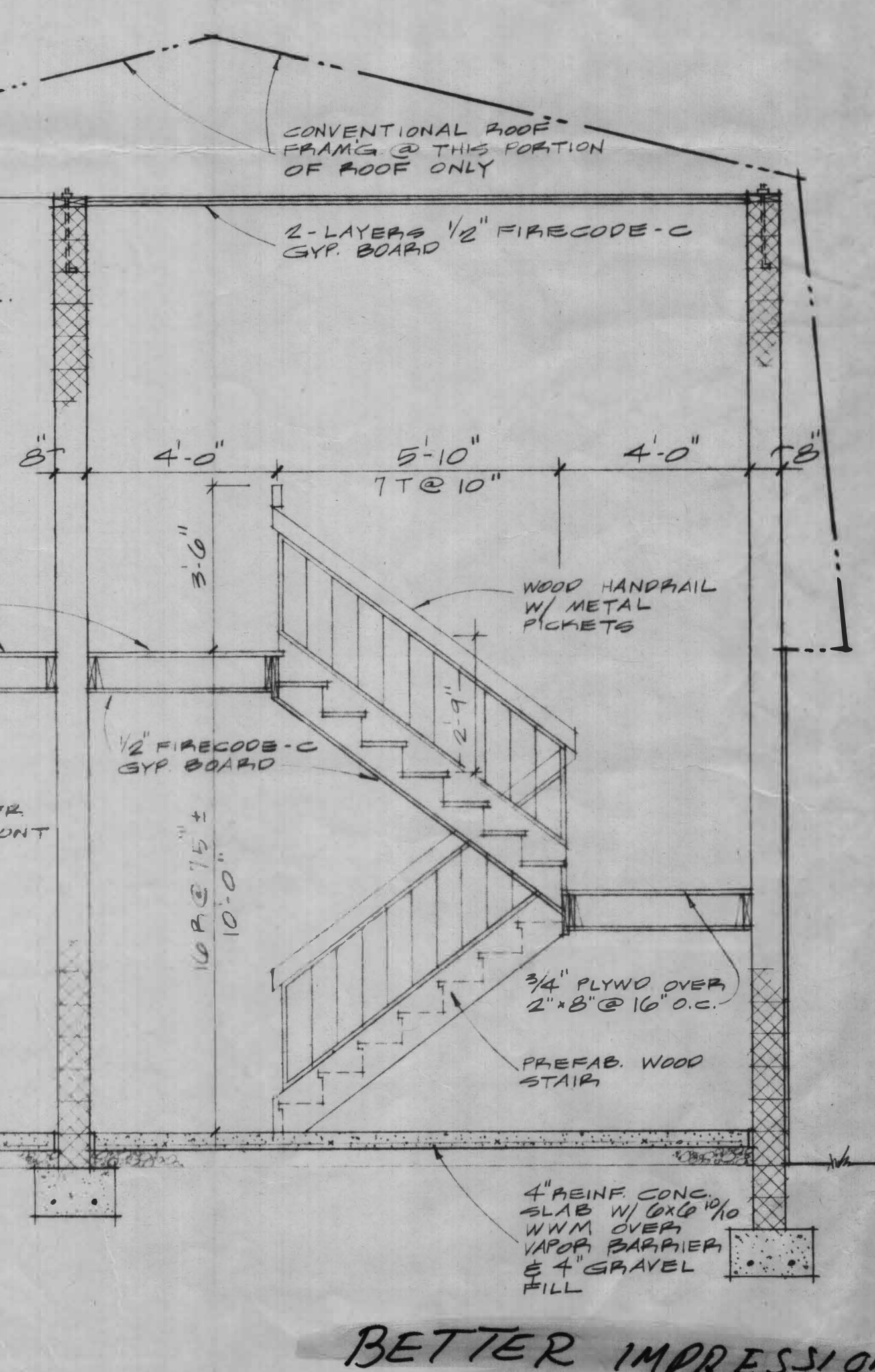
SECTION C 1/2" = 1'-0"
