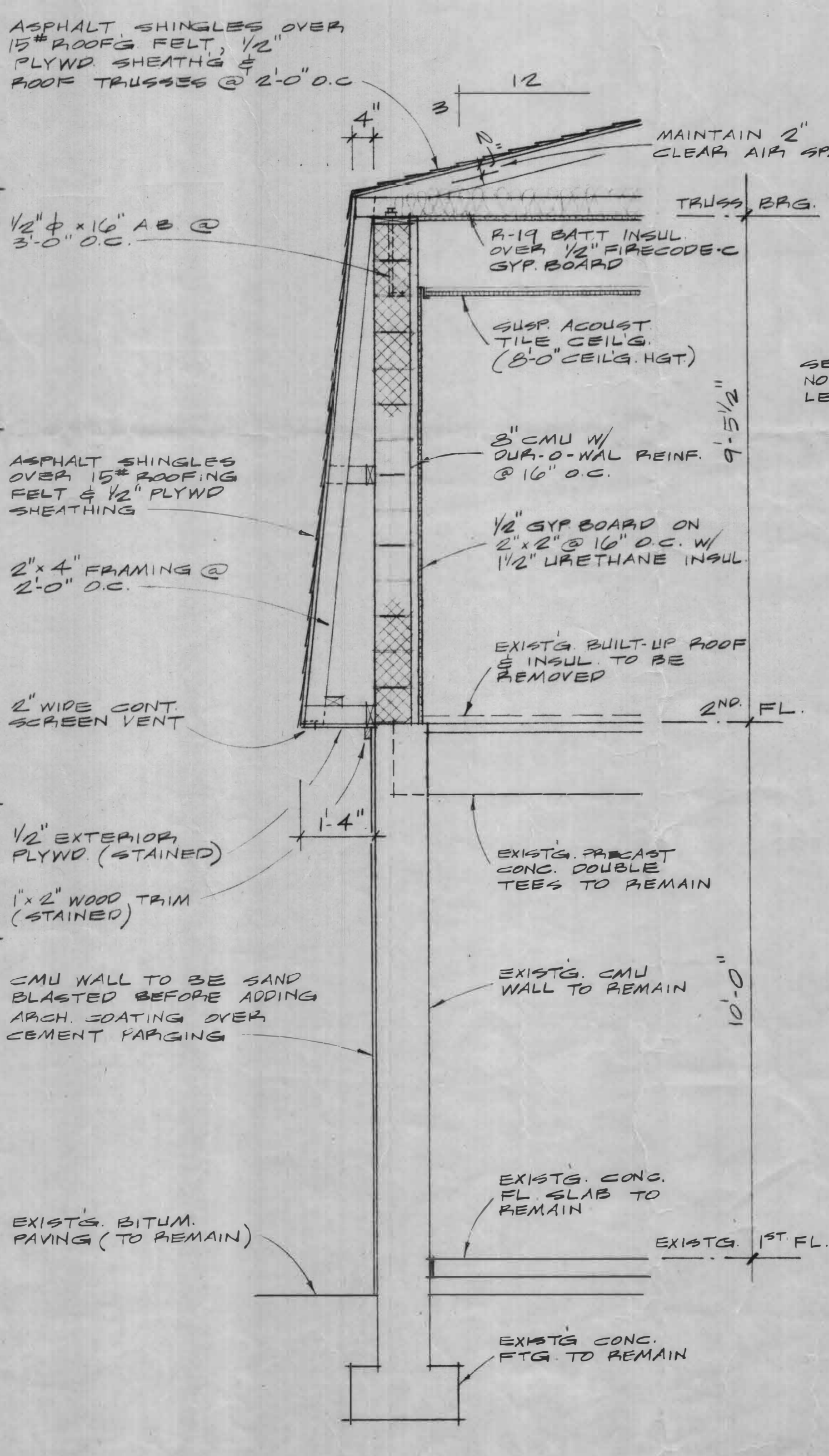
SECTION A 1/2" = 1'-0"
