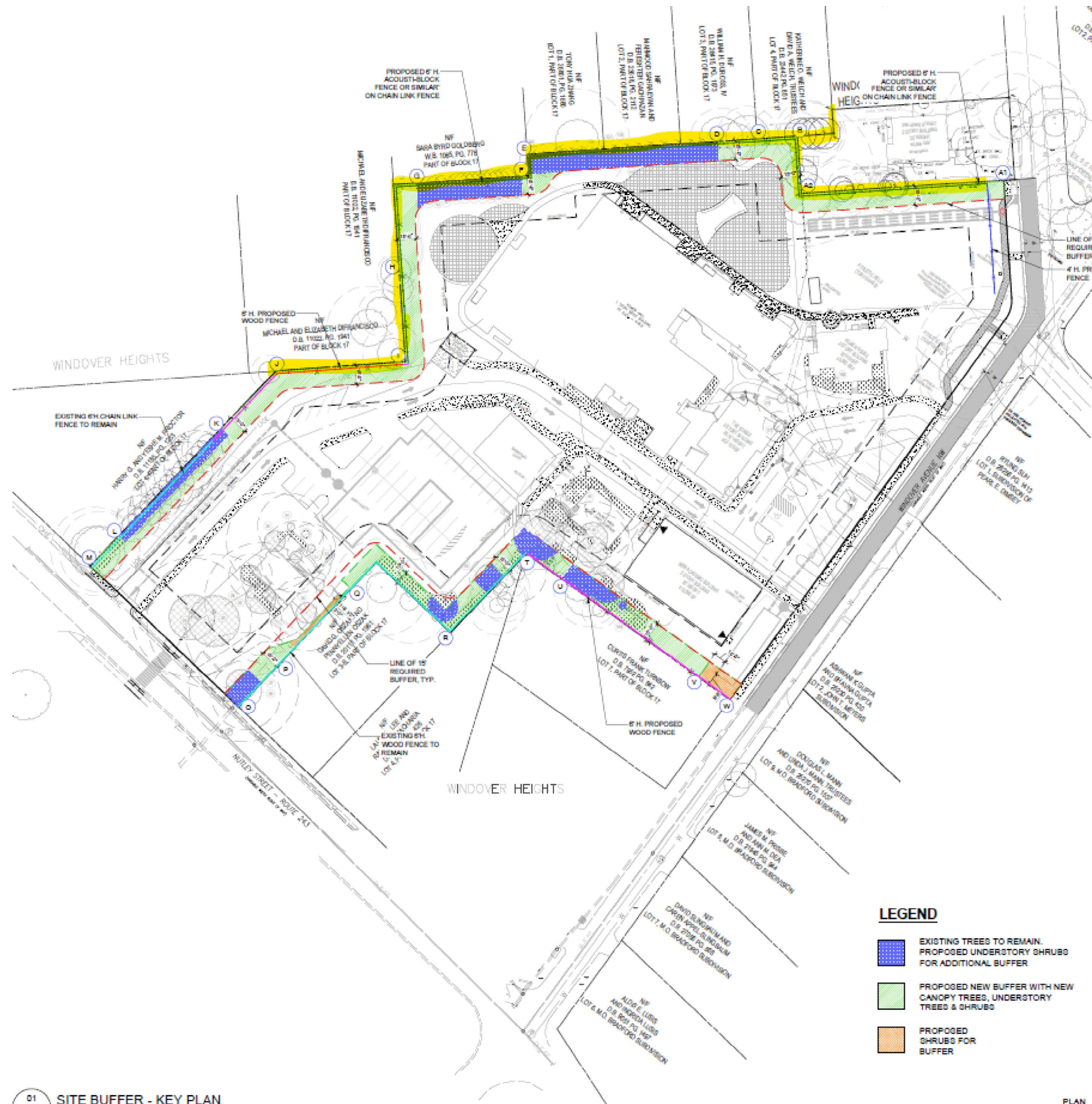
01 SITE BUFFER - KEY PLAN Scale: 1"=40'-0"
