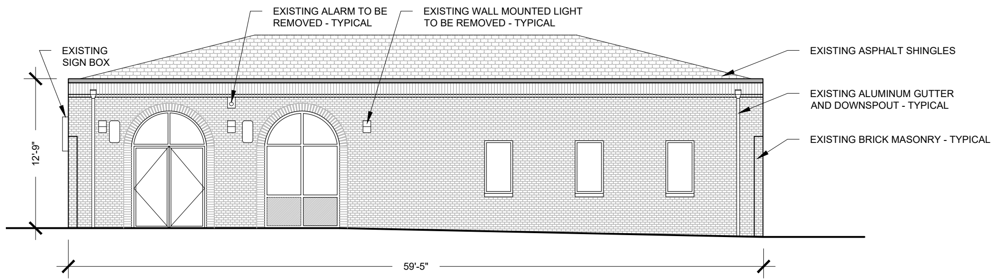
NORTHEAST ELEVATION
