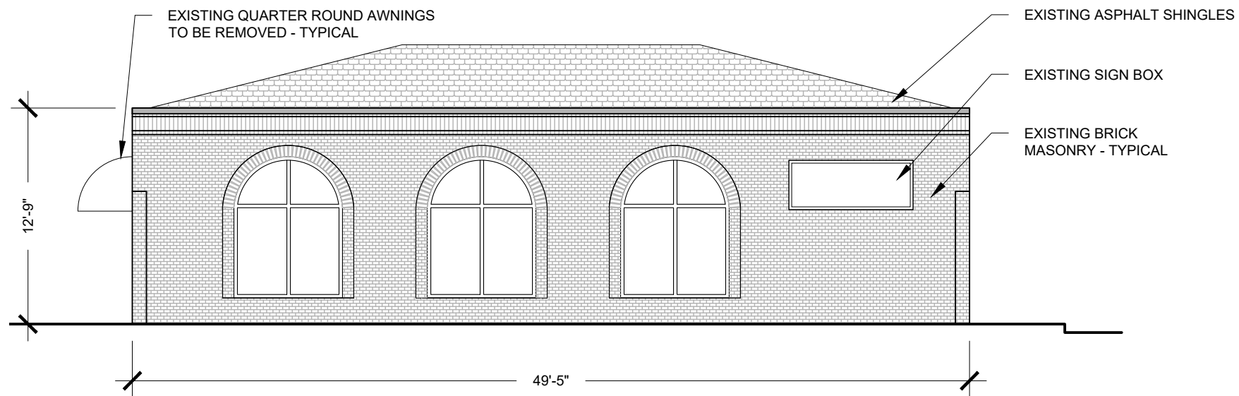
SOUTHEAST ELEVATION
