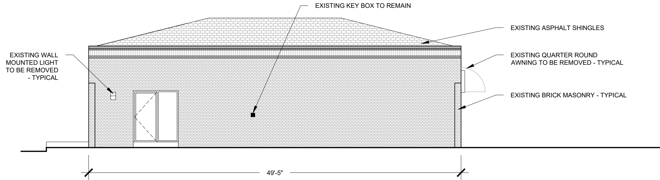
NORTHWEST ELEVATION
