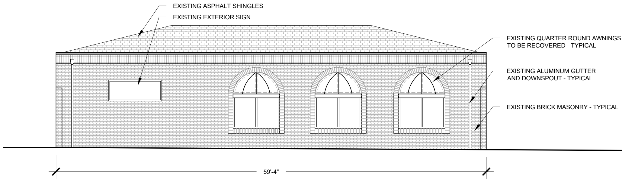
SOUTHWEST ELEVATION
