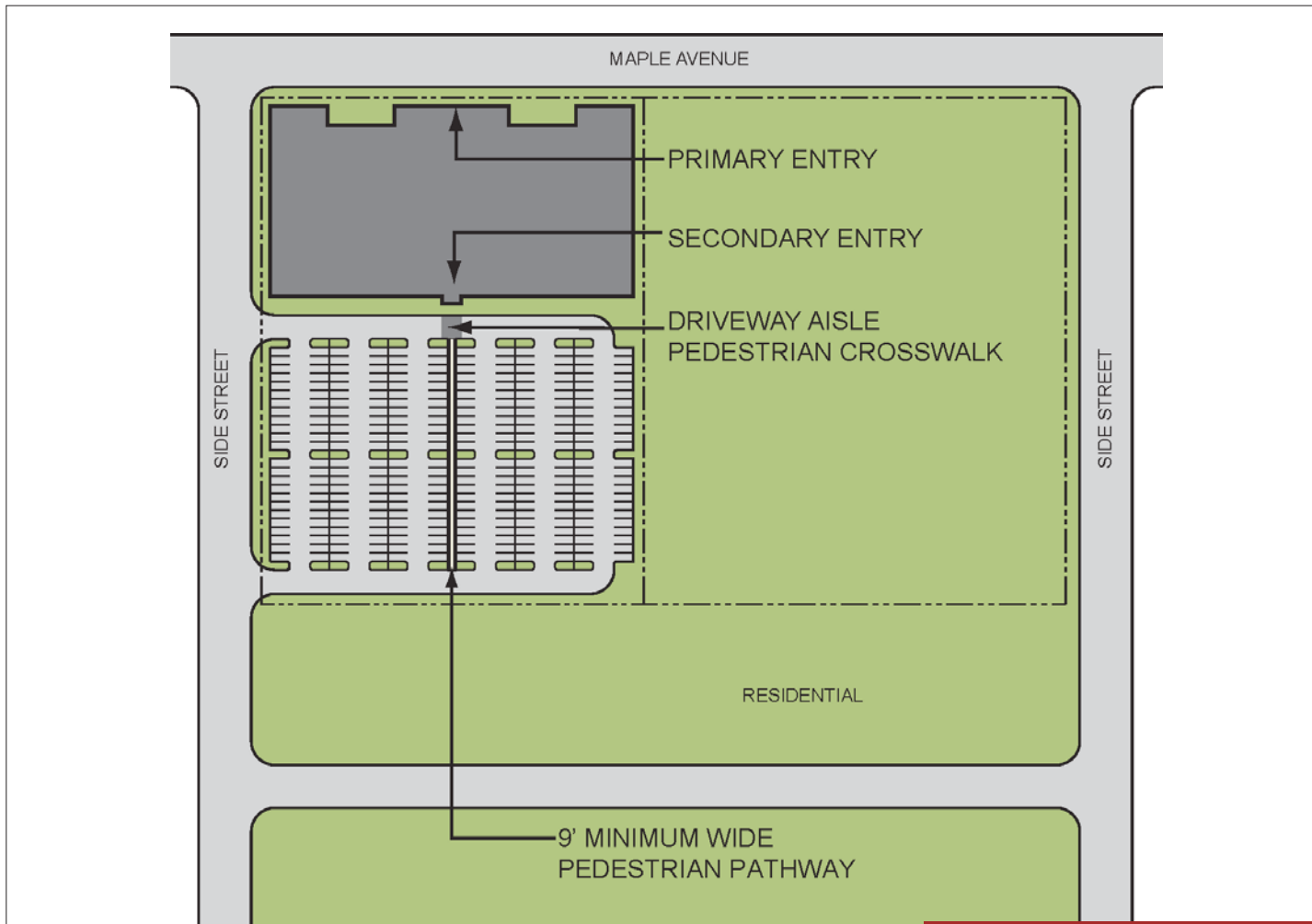
18-95.10.1 Pedestrian Pathways
