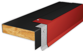
UNA-Edge DRIP EDGE Kynar 500® Finish with and without Continuous Cleat Versions
