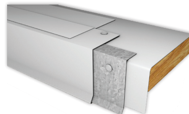
UNA-Edge TPO COATED DRIP EDGE TPO Coated with and without Continuous Cleat Versions
