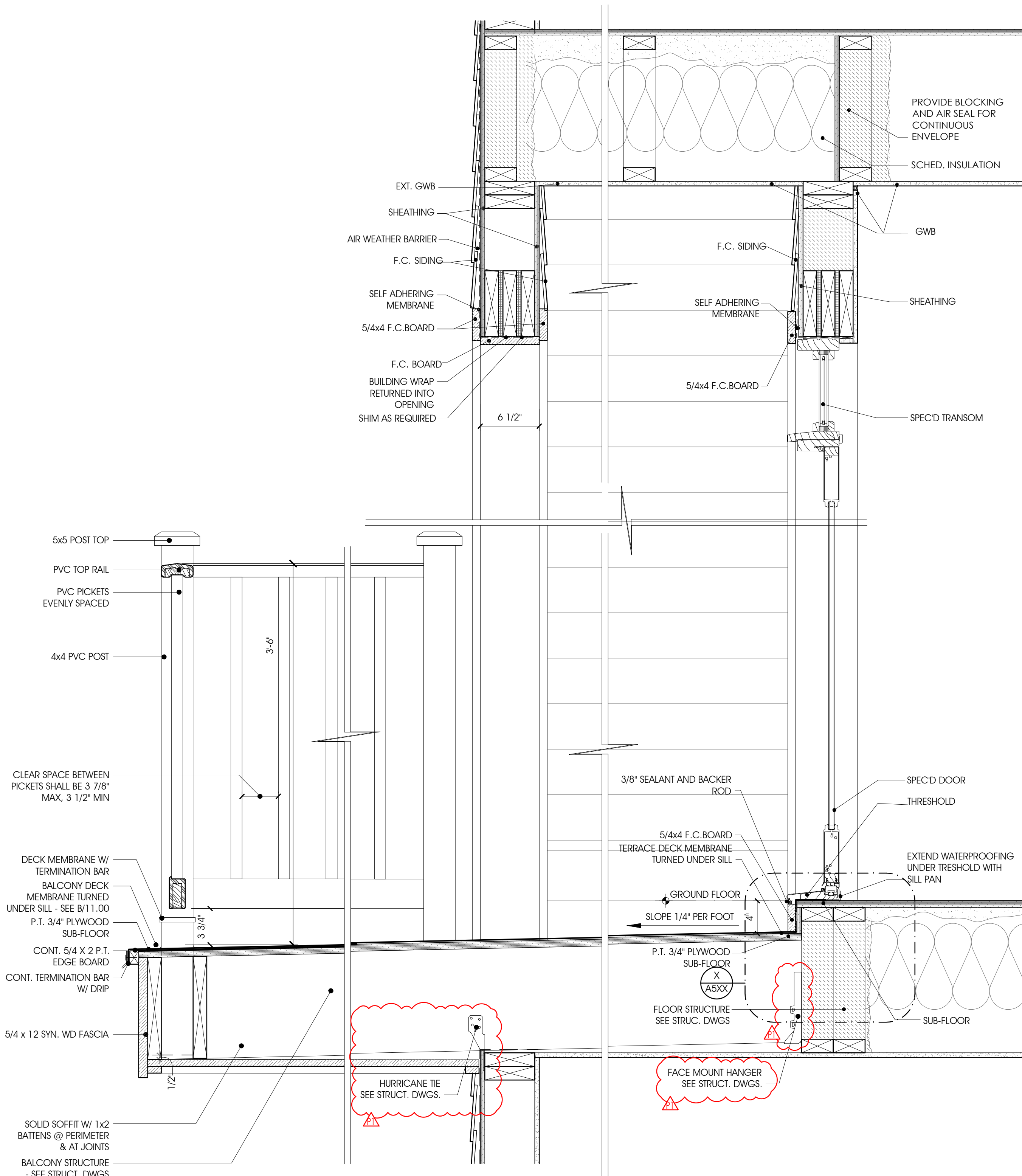
REAR BALCONY DETAIL 1 1/2" = 1'-0"
