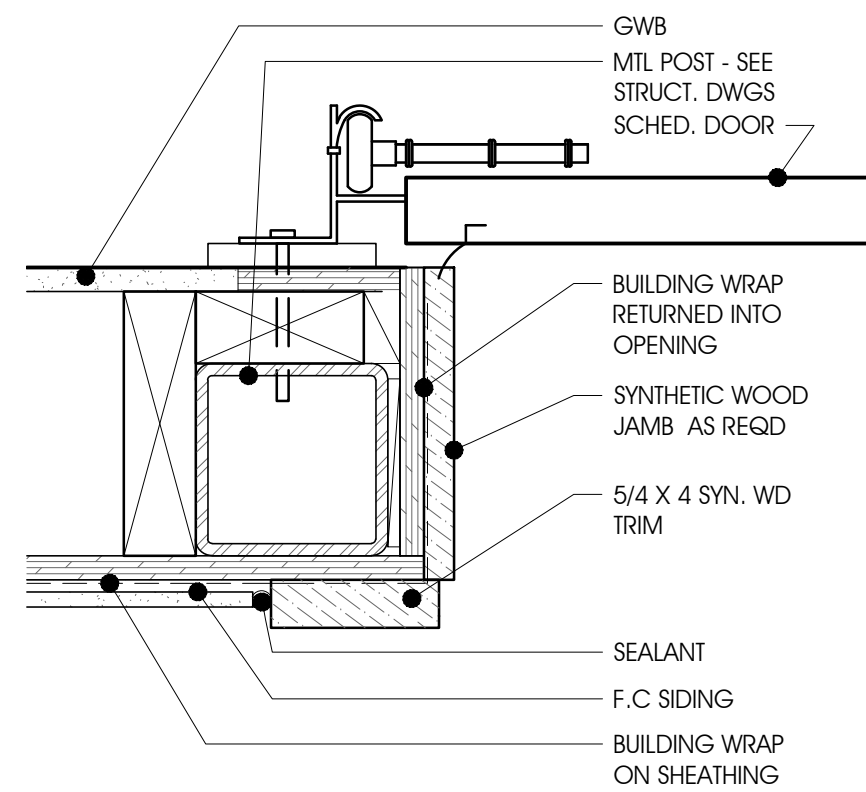
GARAGE DOOR JAMB DETAIL 3" = 1'-0"
