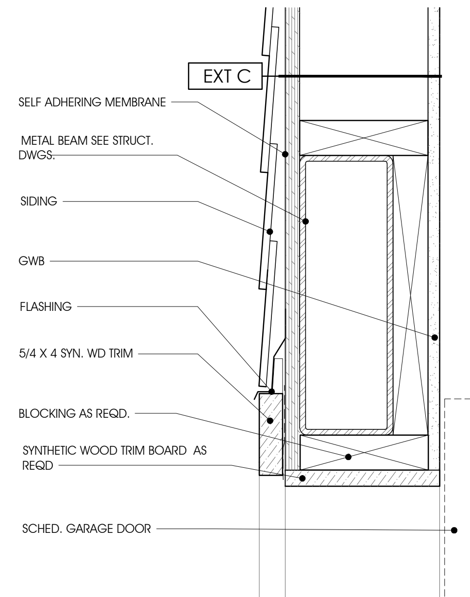
GARAGE DOOR HEAD DETAIL 3" = 1'-0"
