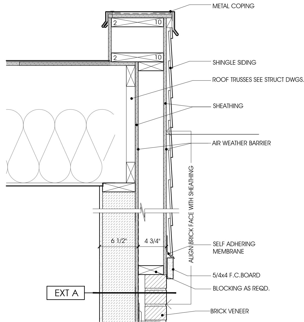
SHINGLE WALL DETAIL AT SIDE ELEVATION 1 1/2" = 1'-0"
