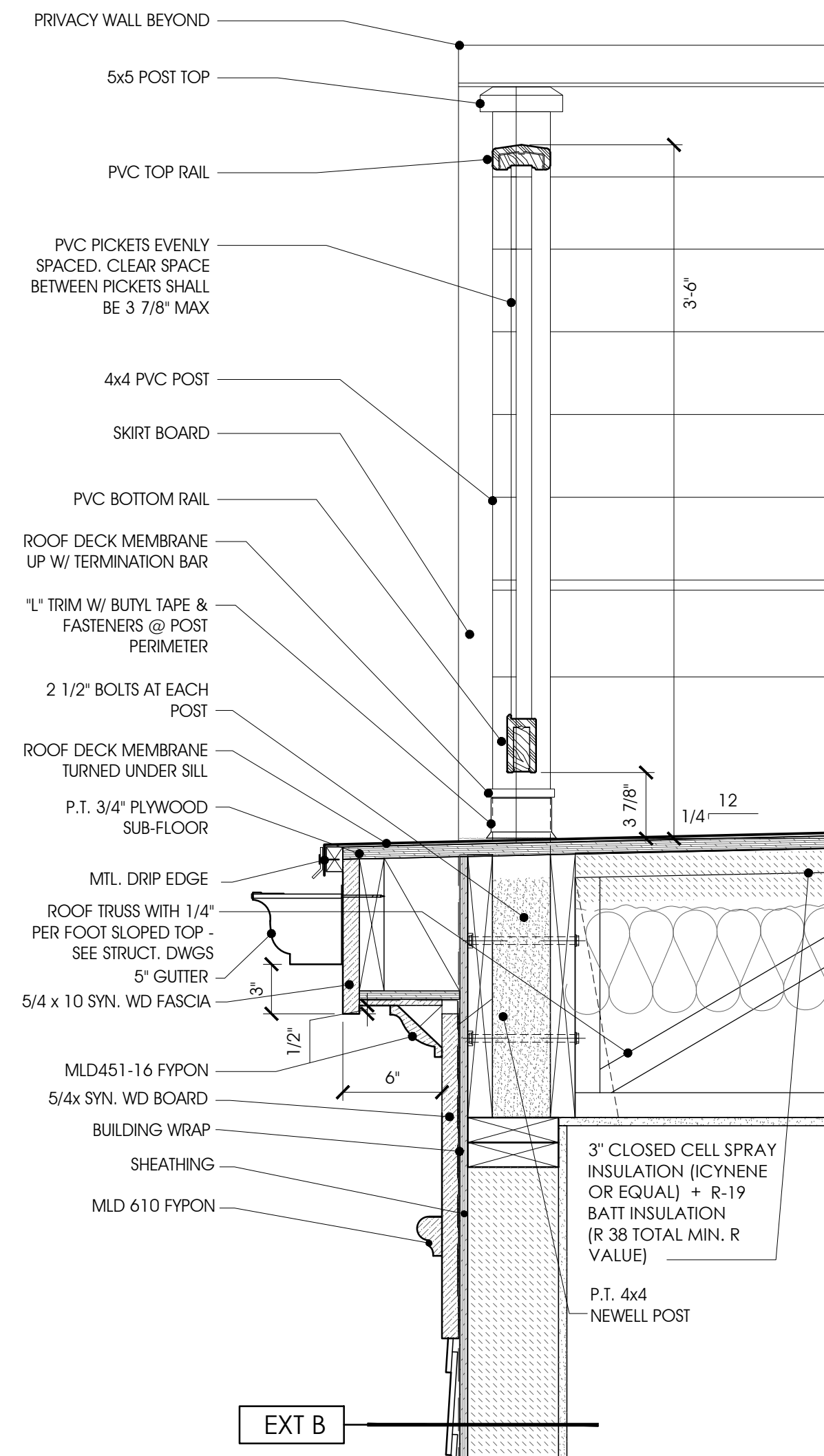
RAILING AT ROOF TERRACE DETAIL 1 1/2" = 1'-0"
