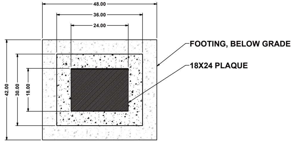
1 PLAN VIEW SCALE 1:12
