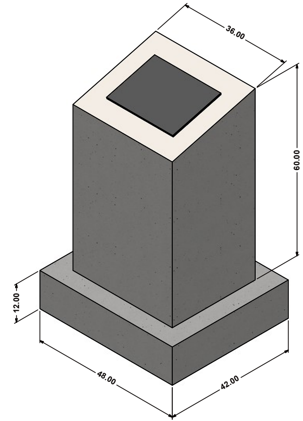
4 ISOMETRIC VIEW SCALE 1:12
