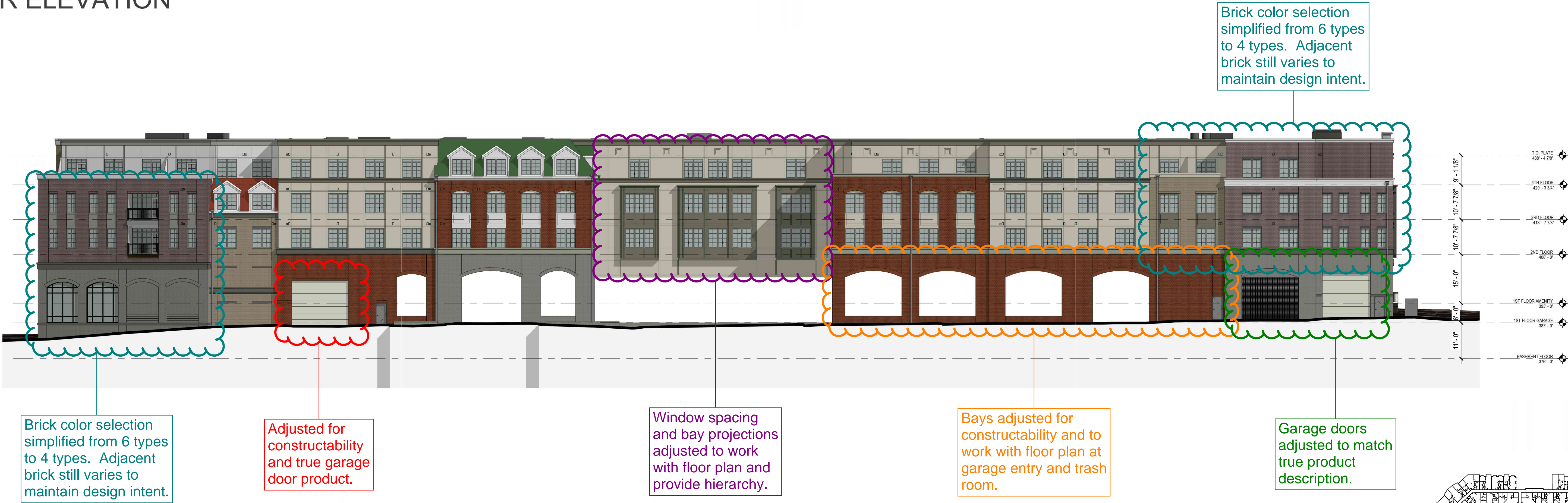
1 - REAR ELEVATION
